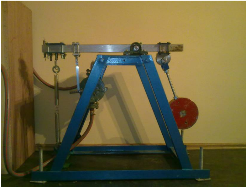
Picture 2. New model of hand water pump with a pendulum
